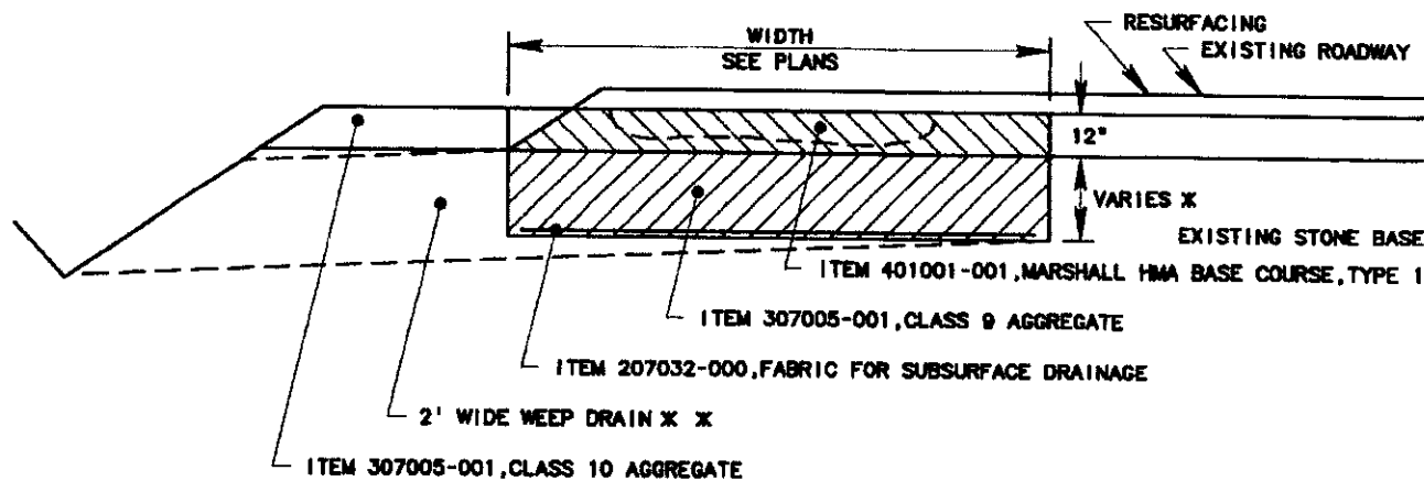
(ELEVATION VIEW)
