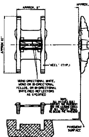
TYPICAL TYPE "P-2" MARKER (ITEM 663022-6)
